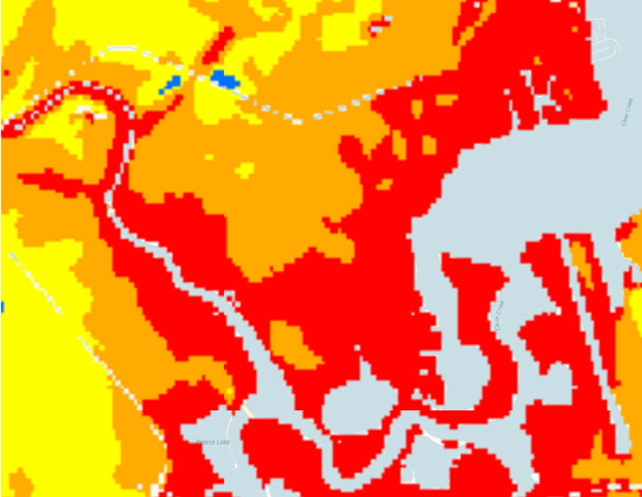
Category 4 (SLOSH MOM) Storm Surge Inundation Height Above Ground up to 3 feet > 3 feet > 6 feet > 9 feet Leveed Area (consult local officials for flood risk)
