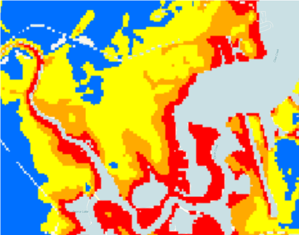
Category 3 (SLOSH MOM) Storm Surge Inundation Height Above Ground ■ up to 3 feet ■ > 3 feet ■ > 6 feet ■ > 9 feet ▨ Leveed Area (consult local officials for flood risk)
