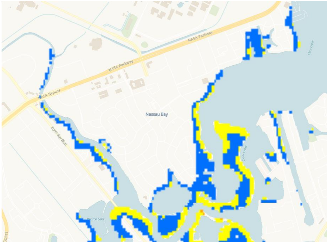
Category 1 (SLOSH MOM) Storm Surge Inundation Height Above Ground
