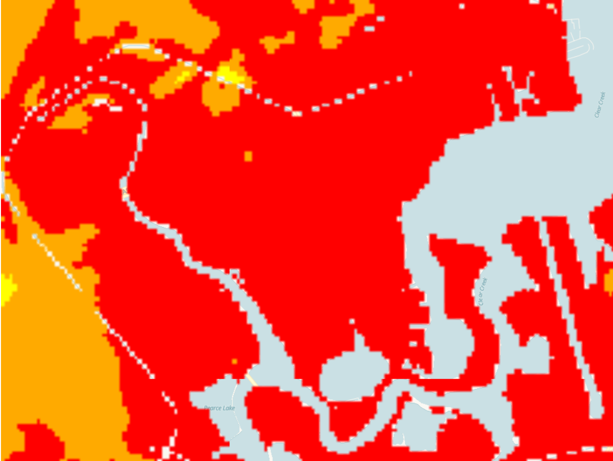
Category 5 (SLOSH MOM) Storm Surge Inundation Height Above Ground ■ up to 3 feet ■ > 3 feet ■ > 6 feet ■ > 9 feet ▨ Leveed Area (consult local officials for flood risk)
