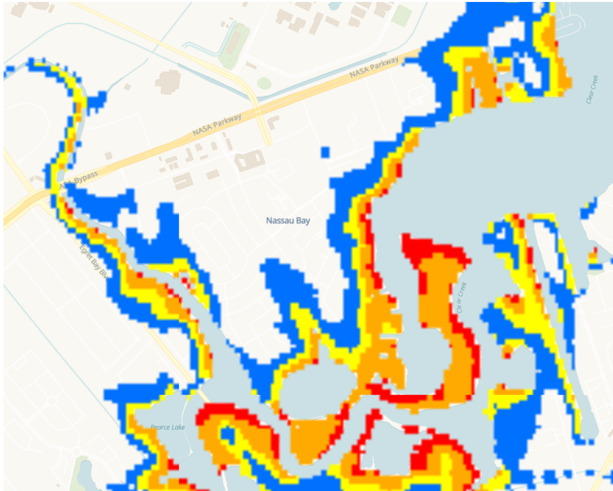
Category 2 (SLOSH MOM) Storm Surge Inundation Height Above Ground
