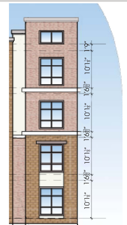
Typical Elevation Dimensions
